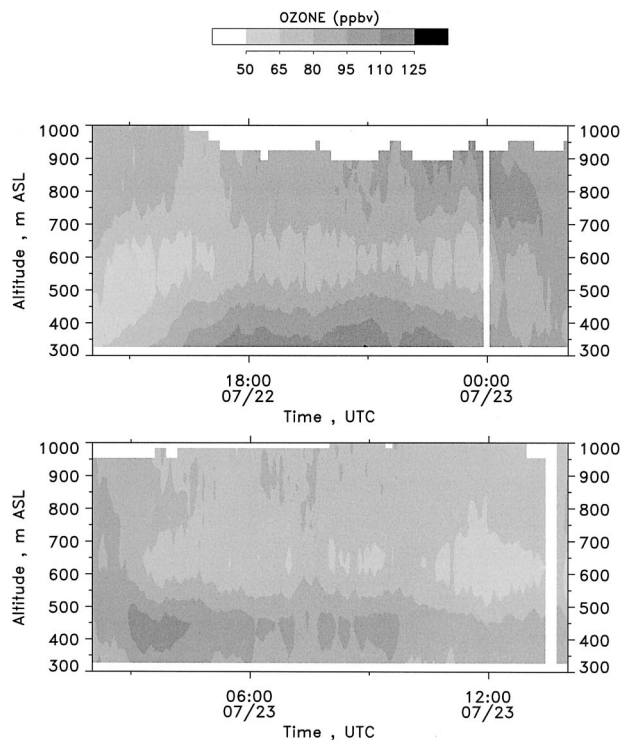
FIG. 9. Ozone concentration observed above the ship on 22 and 23 Jul.
