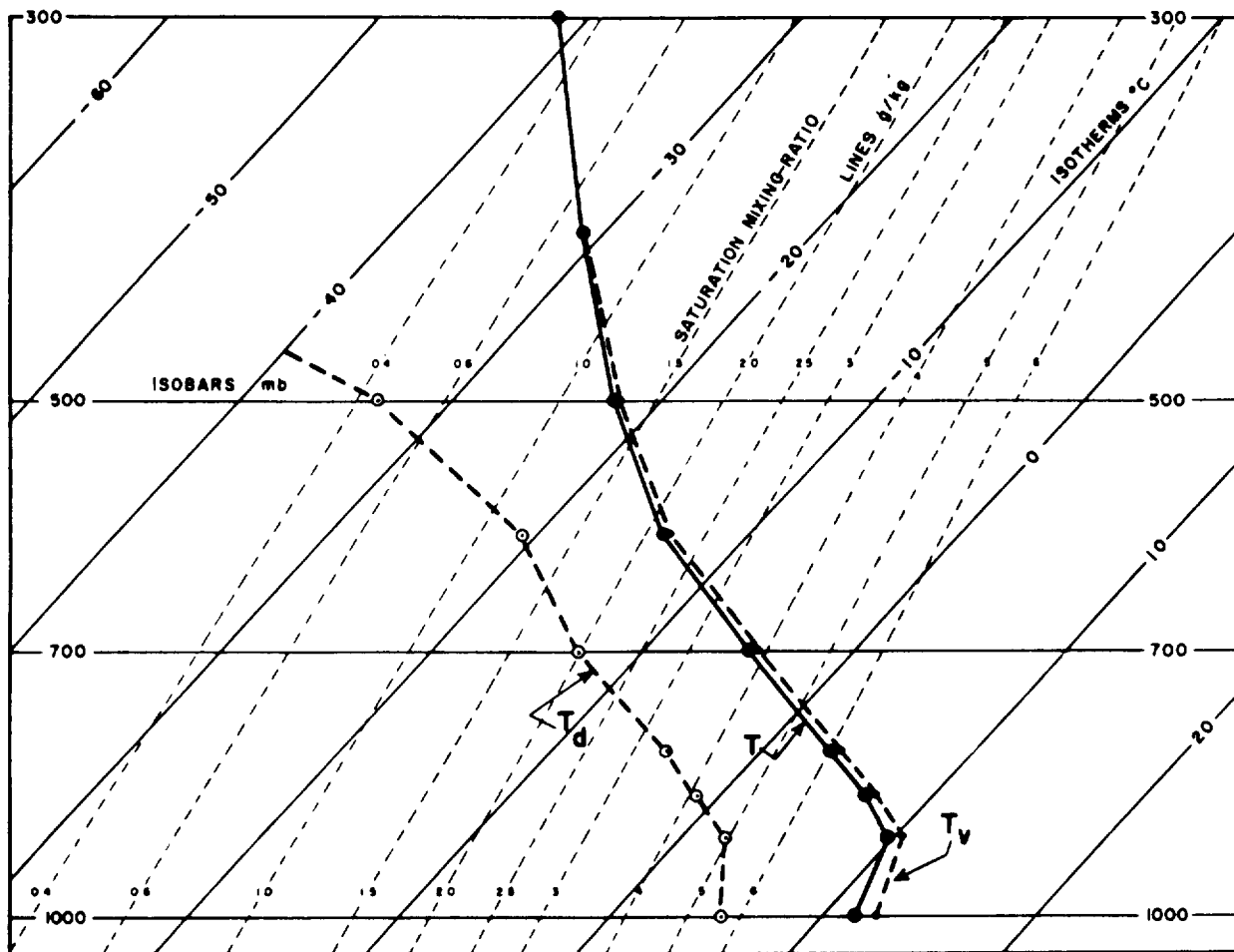
Figure 16. Comparison Between the Observed-Temperature and Virtual-Temperature Curves.
