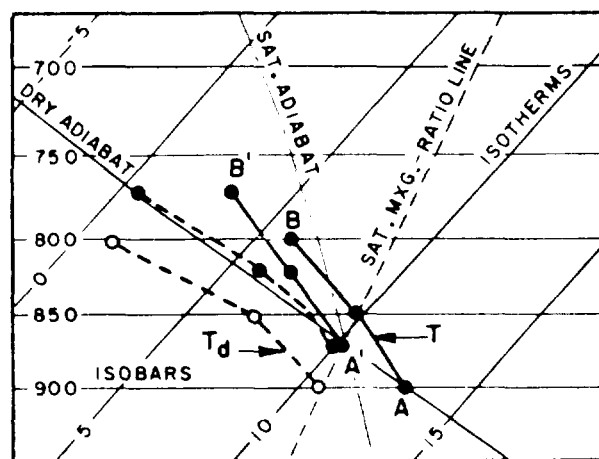
Figure 35b. Effect of Lifting a Conditionally-Unstable Layer on the Release of its Potential Instability.
