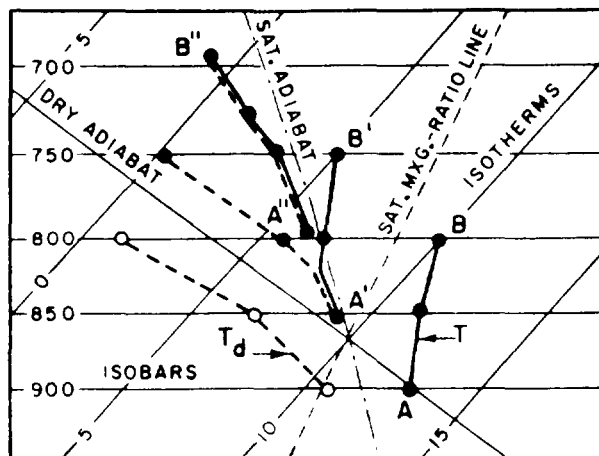
Figure 35a. Effect of Lifting an Absolutely-Stable Layer AB on the Release of its Potential Instability.
