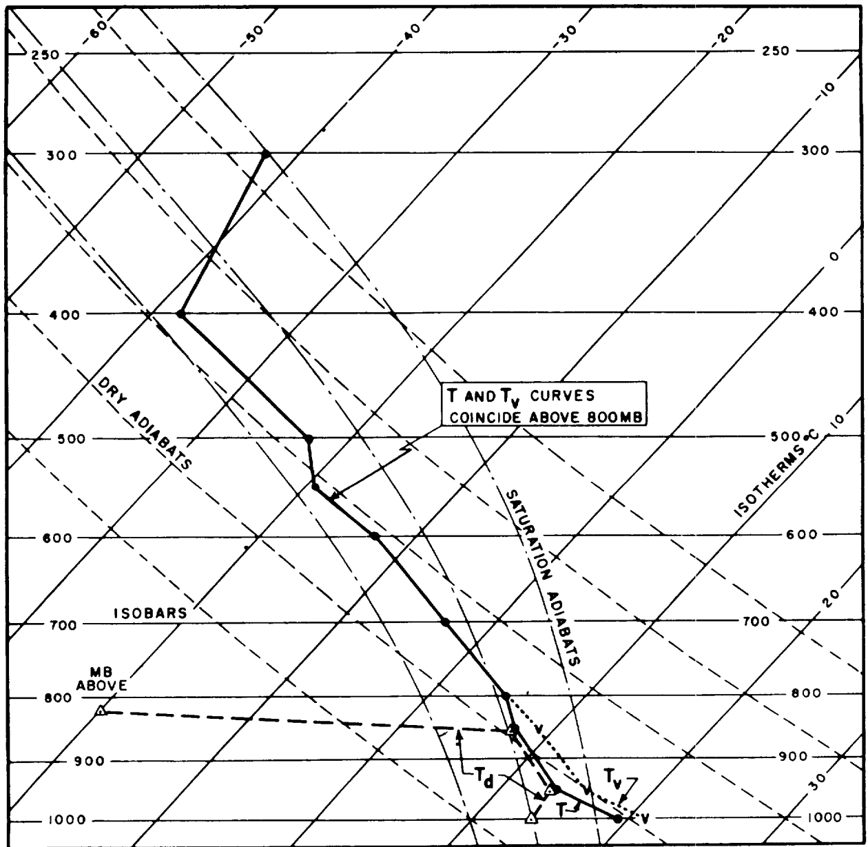
Figure 24. Sample Sounding for Stability Analysis.
